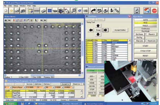
Model LS60 Board sizes to 13.5" x 32" & 96 feeder positions
