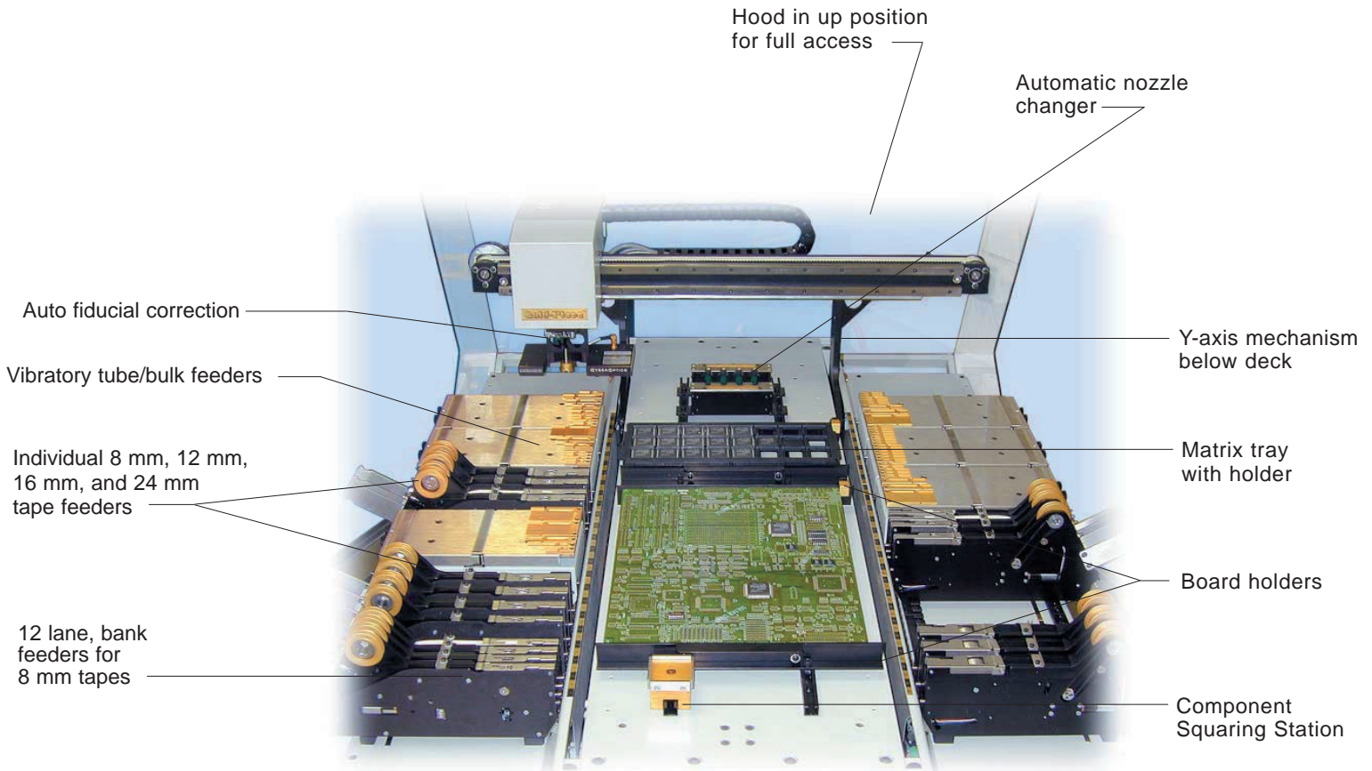
Model LS60 showing easily accessible, unobstructed work deck
