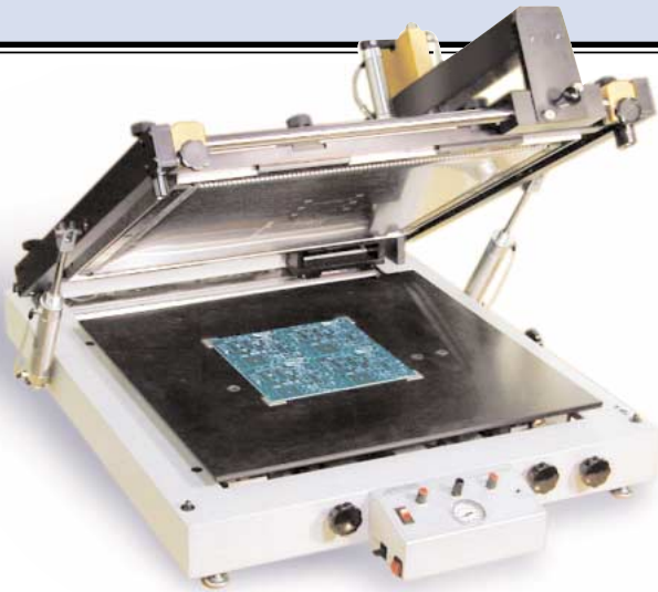
Model SPR-45 semi-automatic stencil printer
